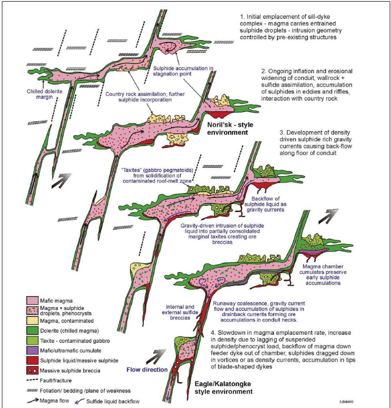
Figure 3. Schematic illustration of an idealised magmatic plumbing system, showing a hypothetical sequence of events leading to the development of Noril'sk style, Eagle–Kalatongke style and Voisey's Bay style mineralisation. (Barnes et al, 2015)
