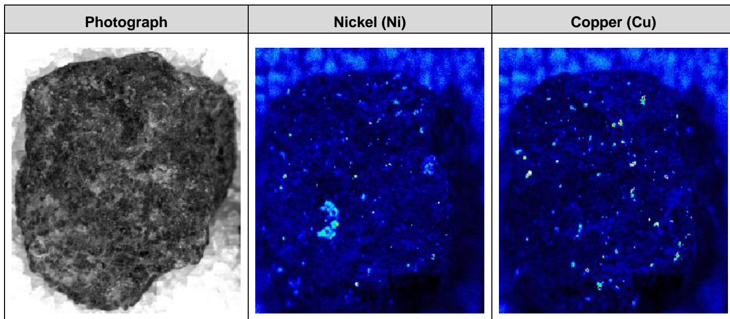
Figure 2. MVR003 (79-80m) photograph (left) and nickel and copper “maps” where bright spots indicate high values. (Field of view approximately 12mm).
